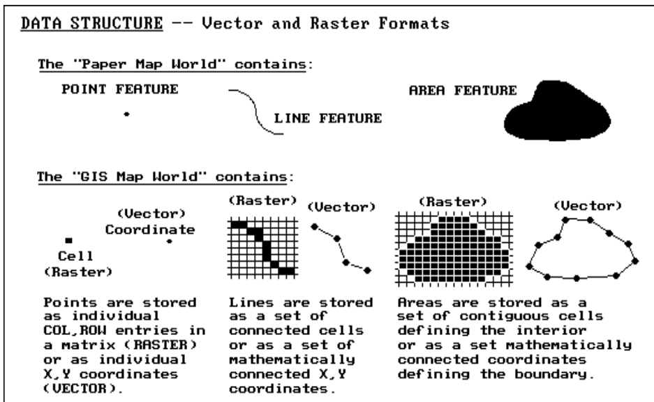
Figure 8.8: Geographic Data Structure
